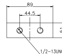
GROUND PAD STAINLESS STEEL
