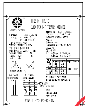
NAMEPLATE
